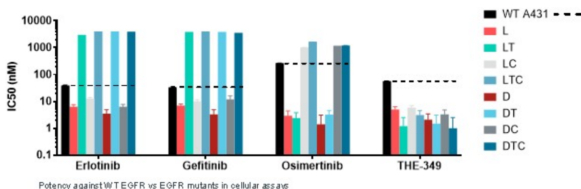
Figure 17. Summary of cellular IC 50 values including control (erlotinib and osimertinib) and THE-349 against wild-type (WT) EGFR and a panel of single- (D, L), double- (DT, DC, LT, LC) and triple- (DTC, LTC) mutant EGFR variants.
