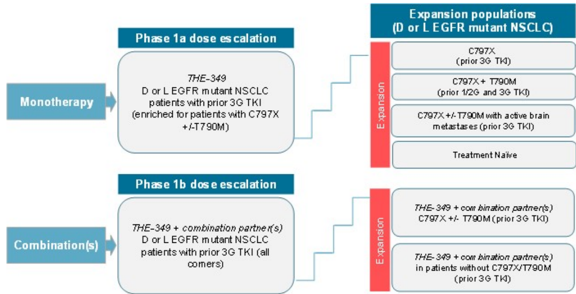
Figure 20. Clinical development plan for THE-349.
