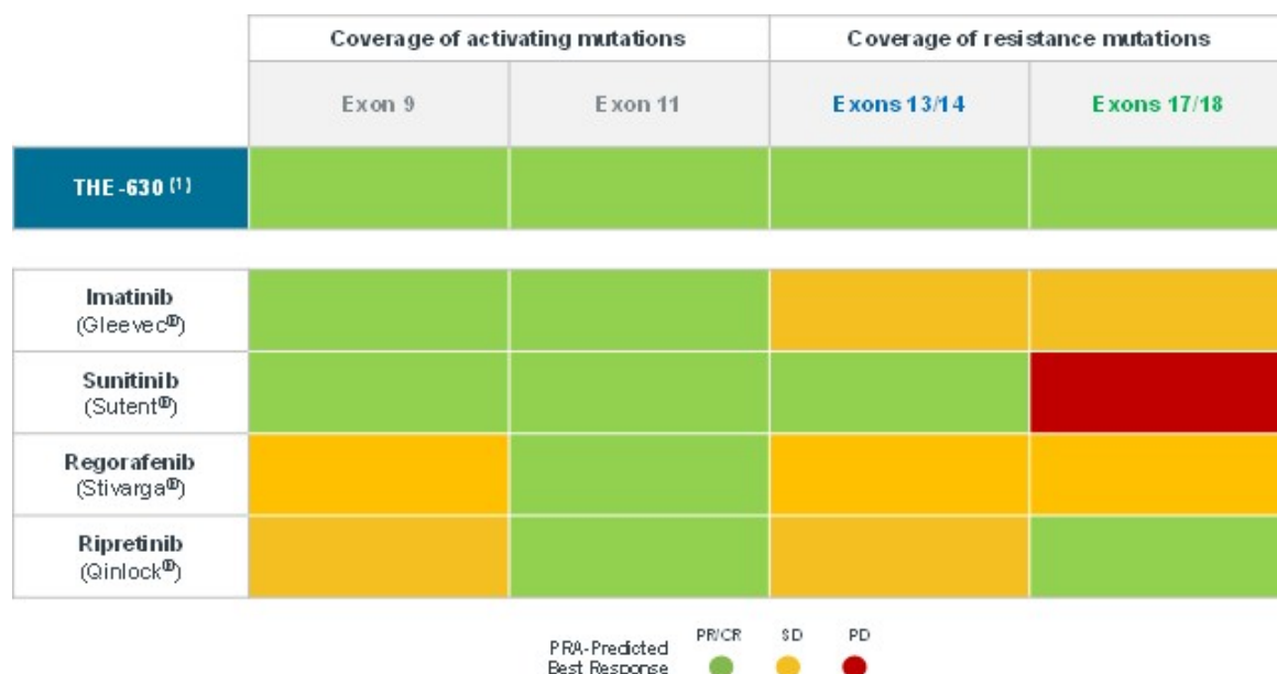
Figure 7. Clinical activity profile predicted by our PRA for benchmark TKIs and THE-630 against all major classes of KIT activating and resistance mutations. PR/CR means partial/complete response; SD means stable disease; PD means progressive disease.
