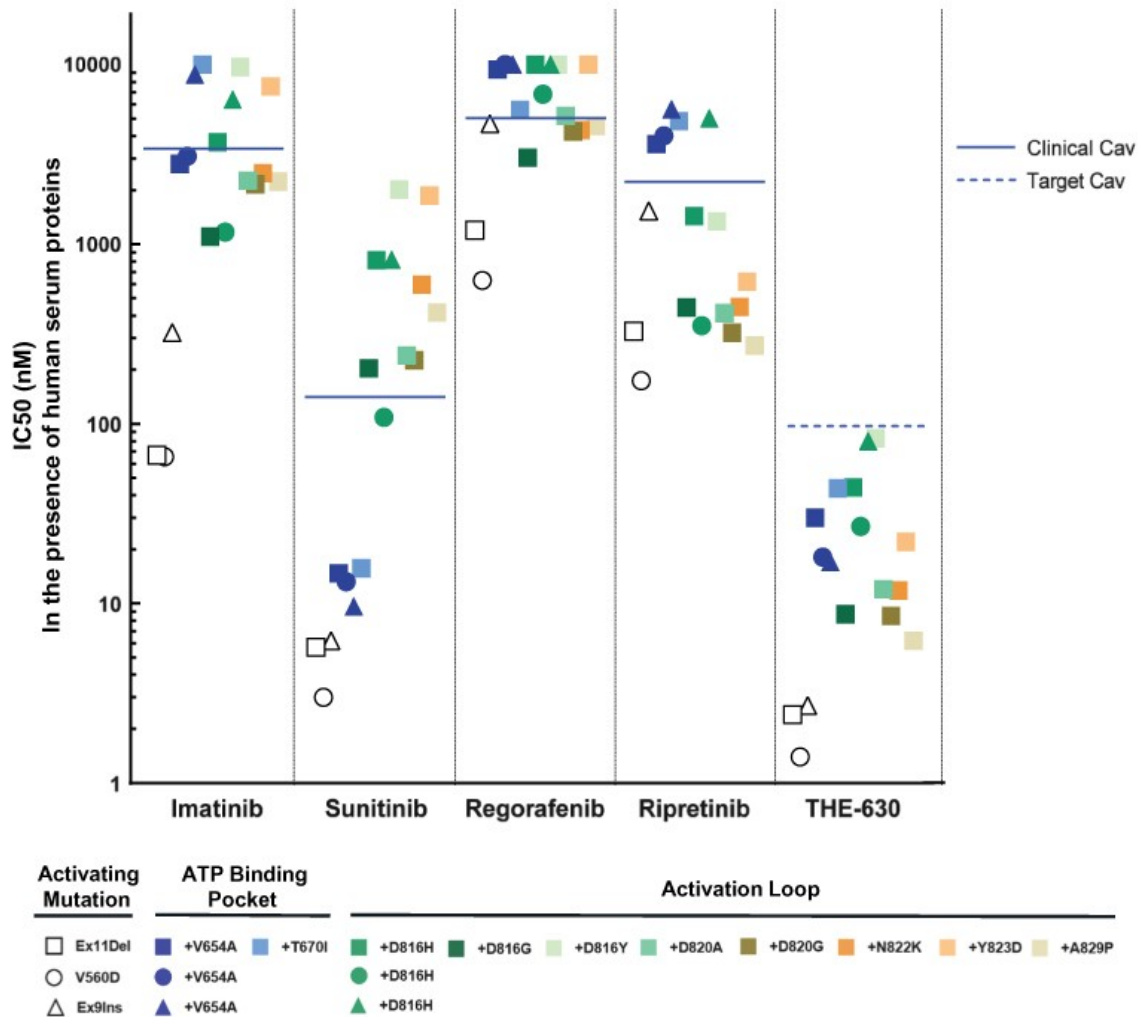
Figure 6. Activity of THE-630 and benchmark TKIs in the PRA of cytotoxicity against KIT activation and resistance mutations showing a broad activity profile. The y-axis shows the IC 50 value range using a log 10 scale.
