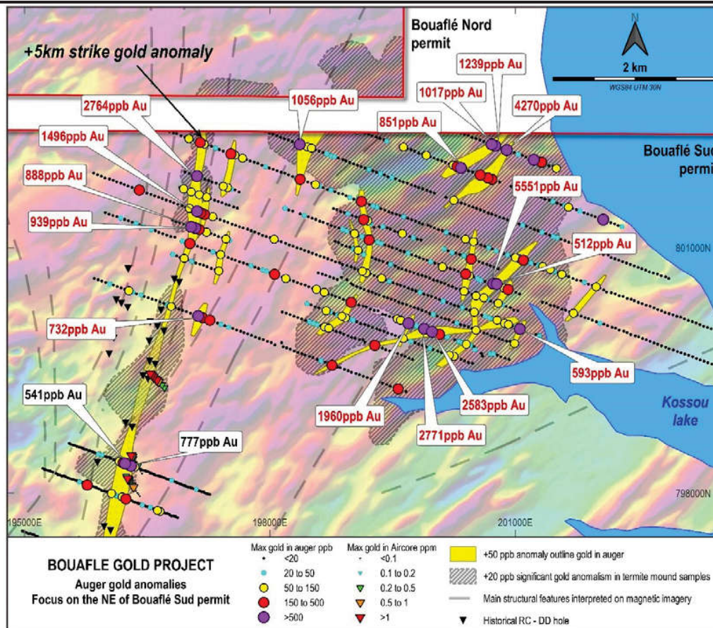
Figure 6 – Auger anomalies at the NE Zone of Bouaflé Sud; magnetic susceptibility imagery as background
