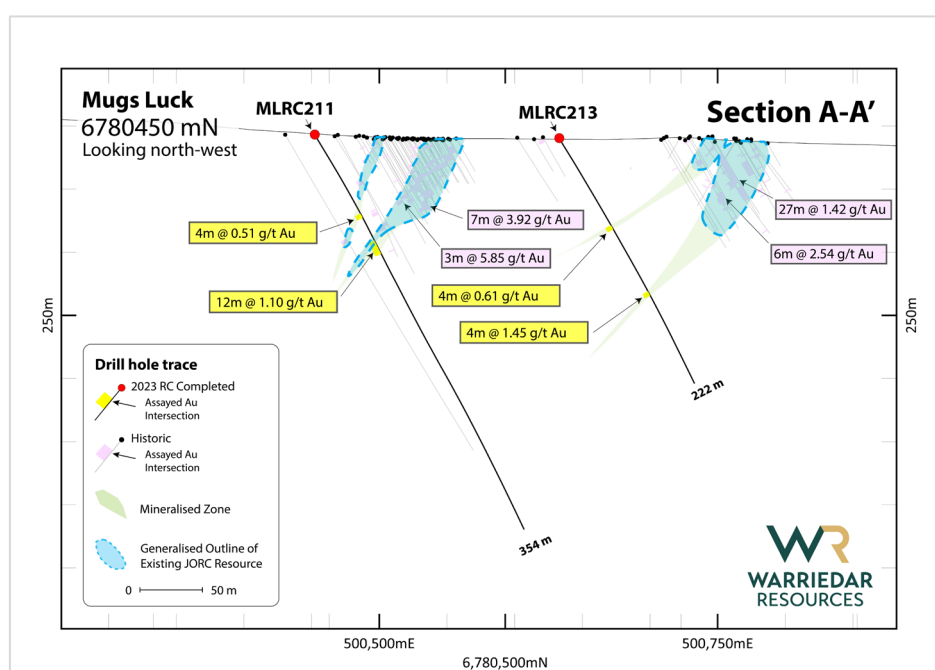
Figure 7: Cross section through the Mugs Luck drilling.
